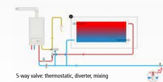
5-way valve: thermostatic, diverter, mixing
